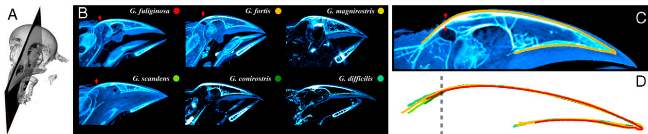
Fig. 2. Midsagittal cuts of three-dimensional reconstructed heads of the different species in Geospiza obtained by Computed Tomography (CT) scans. (A) Example of a three-dimensional reconstruction of a bird skull obtained by CT showing the plane corresponding to a midsagittal cut. (B) Midsagittal cuts obtained from three-dimensional reconstructions of CT scans for the different species in the genus Geospiza . Color dots label the species. Red arrows show the top-most position of the keratin layer indicating that soft tissue is found beyond this point. (C) Zoom of the upper part of the beak of the Medium Ground Finch ( Geospiza fortis ) showing the digitized outline of the bone structure of the upper part of the beak (orange curve). (D) Outlines of the bone structure of the upper part of the beak for the different species shown in B collapsed via a nonuniform scaling transformation. The dashed line indicates the position of the divergence point (see main text).
