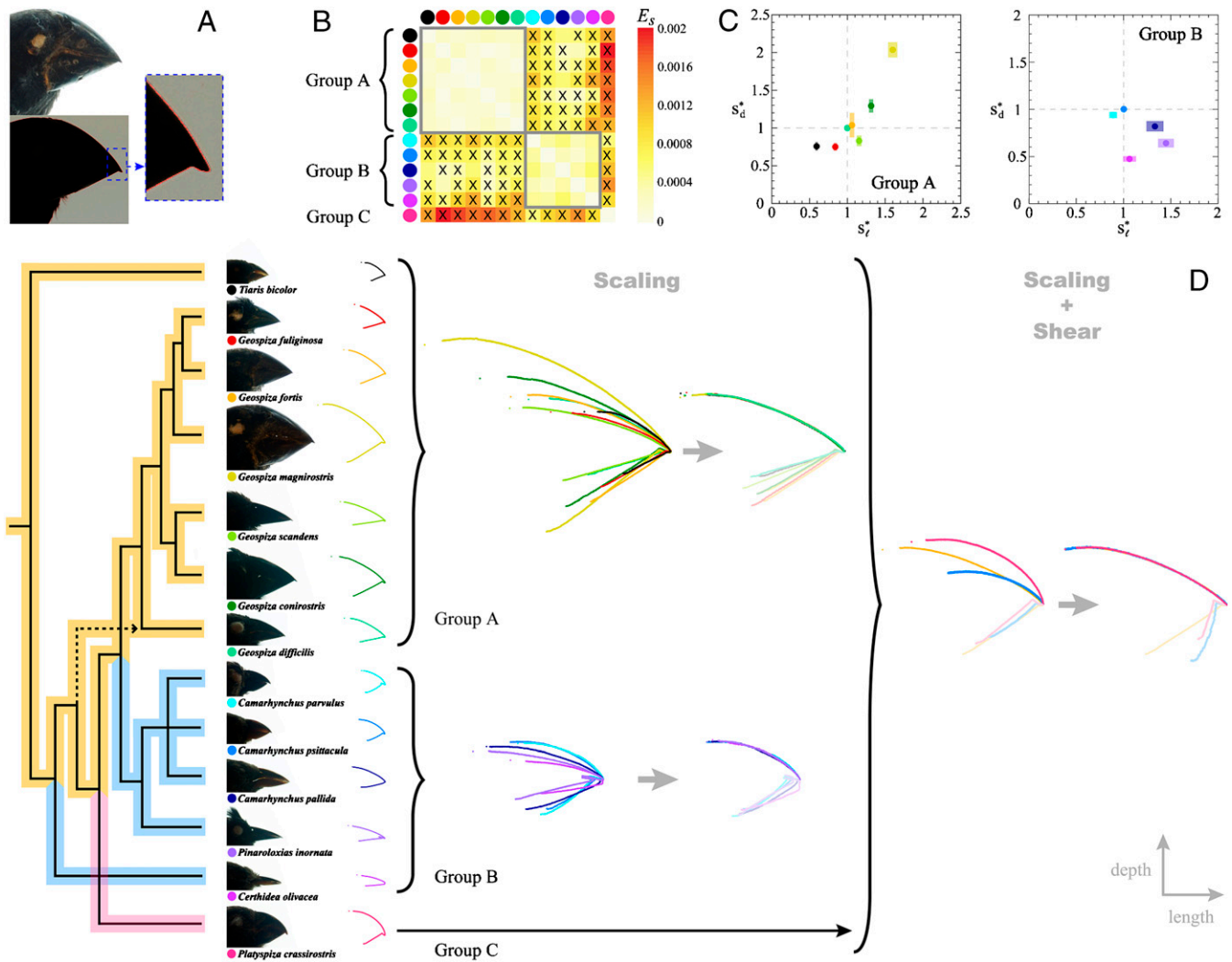
Fig. 1. Geometric relations among the beaks of Darwin's Finches. (A) Example of digitization of a beak profile: (Top) Normal exposure picture of a museum specimen of the Large Ground Finch ( Geospiza magnirostris ). (Bottom) Underexposed picture of the same bird, with the outline of the bird silhouette traced in red. The zoomed region shows that the beak outline can be traced at pixel accuracy (Pixel size, 40 μm). See SI Text for further details. (B) Heat map resulting from all pairwise comparisons of beak shapes. The colored dots indicate the species, as labeled in D. Crosses (X) indicate pairs of species whose beaks do not collapse via scaling transformations, as there was no minimum in the defined measures E_s and E_d as a function of the scaling factors. Conversely, comparisons not marked with an X indicate that there was a minimum. In this case the plotted color represents the residual E_s(s_r^*, s_d^*) . The same results are obtained for the residuals E_d(s_r^*, s_d^*) . For those pairs marked with an X the plotted color indicates the minimal value of E_s in the range of scaling factors that the experimental error allows to search for. The existence of a minimum in E_s and E_d is not a guarantee of a collapse of the shapes; large values of the residuals are indicative of a lack of collapse. The beak shapes of all species in the genus Geospiza and that of the Blackfaced Grassquit ( Tiaris bicolor ) can be related through scaling transformations (Group A); the beak shapes of Tree ( Camarhynchus ), Cocos ( Pinaroloxias inornata ), and Warbler ( Certhidea ) Finches are also related to each other through scaling transformations (Group B); the beak shape of the Vegetarian Finch ( Platyspiza crassirostris —Group C) cannot be collapsed on any other shape through scaling alone. (C) Scaling factors (obtained by minimization of the measures E_s and E_d ) that allow the collapse of the beak shapes of the species in groups A and B. The reference beak to which the scaling factors are referred to is arbitrary and chosen to be the Sharp-beaked Finch ( Geospiza difficilis ) in group A and the Small Tree Finch ( Camarhynchus parvulus ) in group B. (D) From left to right: Darwin's Finches phylogeny modified from Ref. (18) and colored according to the morphological groups obtained with scaling transformations (Group A—orange; Group B—blue; Group C—pink); Lateral pictures of museum specimens of Darwin's Finches and also the Blackfaced Grassquit (color dots label the species); Digitized beak shape profiles (the color of the shape profile indicates the species); Group structure under scaling transformations: (left) untransformed shapes and (right) shapes collapsed onto a common shape via scaling transformations with the scaling factors in C; Collapse of group shapes onto a common shape via a composition of shear (along the depth axis) and scaling transformations. We note that some of the Sharp-Beaked Finch populations are phylogenetically basal either only to the Geospiza Ground Finches or to Cocos and Vegetarian Finches (but not Warbler Finches) but share the group beak shape with both Geospiza and Grassquit. See Methods and the SI Text for a detailed description of the analysis.
