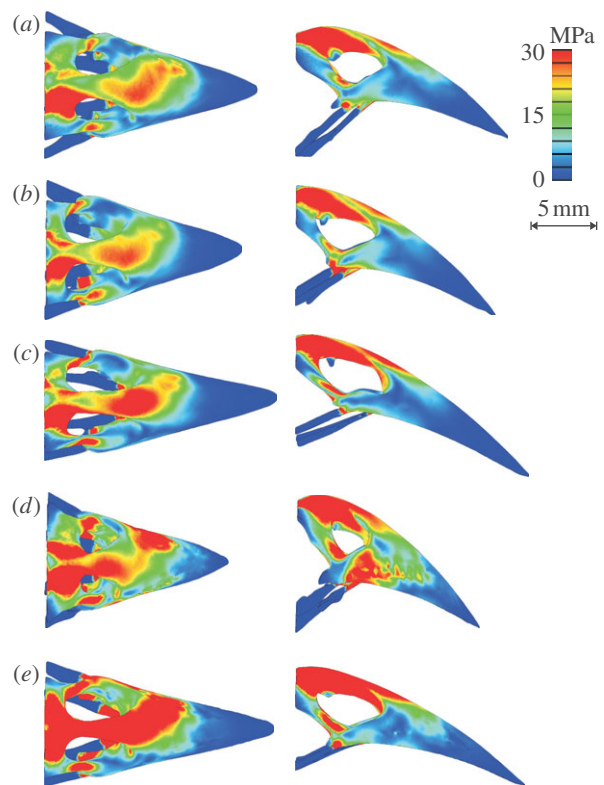
Figure 3. Output of a finite-element simulation, in which beak surface area of the five species of ground finch was scaled to a common surface area (that of G. fortis ) prior to calculations, and in which the input force calculated for G. fortis was applied to all species. This simulation enables the evaluation of the effects of beak shape on stress distribution. The relatively long and slender beaked G. scandens and G. difficilis showed disproportional increases in the magnitude of the von Mises stress and the distribution of areas with high stress (table 1). (a) G. fortis , (b) G. fuliginosa , (c) G. scandens , (d) G. magnirostris , and (e) G. difficilis .
