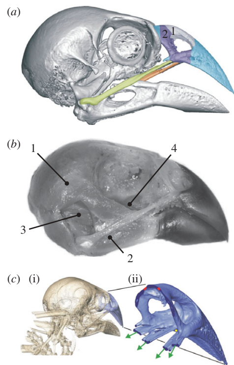
Figure 1. Schematic overview of the model derivation and methods. (a) Lateral view of a three-dimensional reconstruction of the skull of a medium ground finch ( G. fortis ) based on micro-CT scans. When birds bite, forces are transmitted by the jaw muscles to the upper beak (blue) via the jugal bones (green) and the pterygoid–palatine complex (orange). The coloured zone labelled 1 represents the dorsal nasal region, and the zone labelled 2 represents the maxillary process of the nasal bone. (b) Photograph of the head of a G. fortis specimen, skin removed, illustrating the major jaw closing muscles. The external adductor muscles (1, 2) and the m. pseudotemporalis (3) transmit force to the upper beak through the jugal bone. The pterygoideus muscles (4) directly pull the upper beak downward through the pterygoid–palatine complex. (c) Posterior oblique view of (i) the head and (ii) upper beak of a G. fortis , illustrating loadings and constraints used in the finite-element models. Red zones indicate the dorsal constraints on the rotating fixed elements, (i) the yellow circle indicates the bite point and green arrows indicate the orientation of the load acting on the jugals and palatines.
