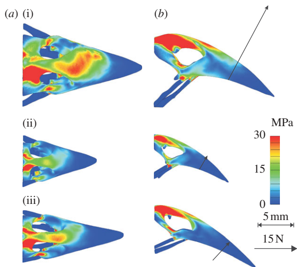
Figure 2. Output of finite-element analyses performed for three different species of ground finches ( Geospiza ) for which specimens were available for dissection. Input forces were calculated from muscle mass and fibre length measurements. Colours indicate calculated resultant von Mises stresses on the beak in (a) dorsal and (b) lateral views: (i) G. fortis , (ii) G. fuliginosa , and (iii) G. scandens . Warmer colours depict higher stresses. For all species, maximum stress concentration occurs at the posterior part of the nasal bone, posterior to the nasal aperture (zone 1 in figure 1a), and within the maxillary processes of the nasal bone (zone 2 in figure 1a). Arrows depict calculated bite forces.
